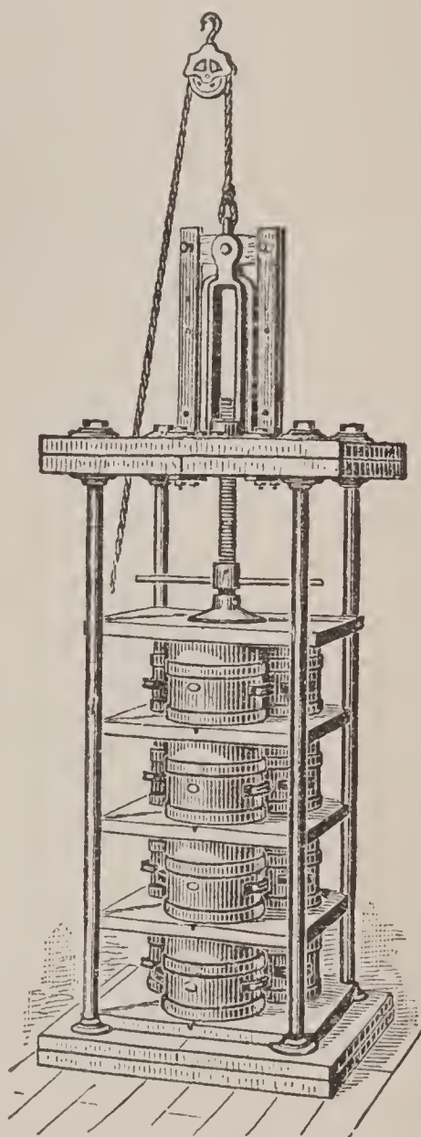
FIG. 422. — Upright gang-press.
