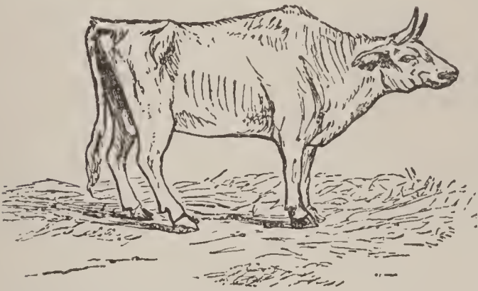
FIG. 426. — Epizootic pleuro-pneumonia.
