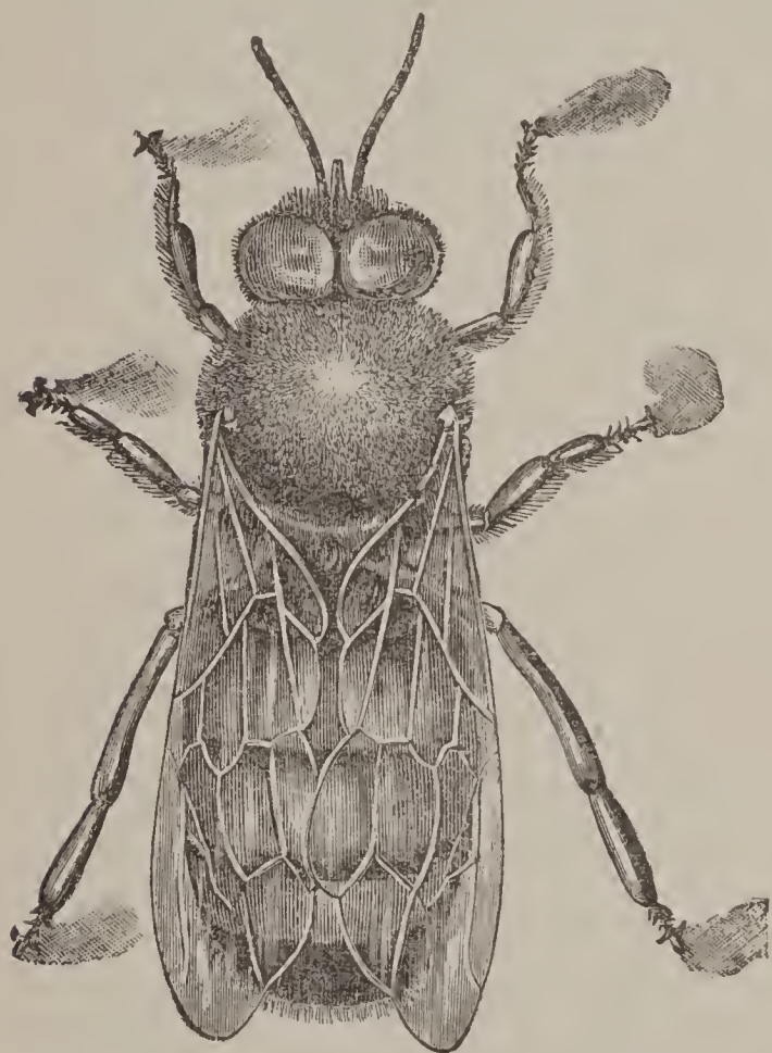
FIG. 586. — Drone bee.
