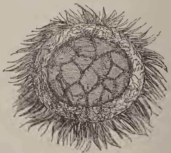
FIG. 462. — Ringworm.
