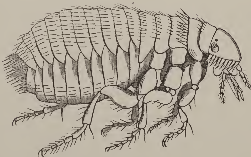
FIG. 584. — Cat-flea, magnified.
