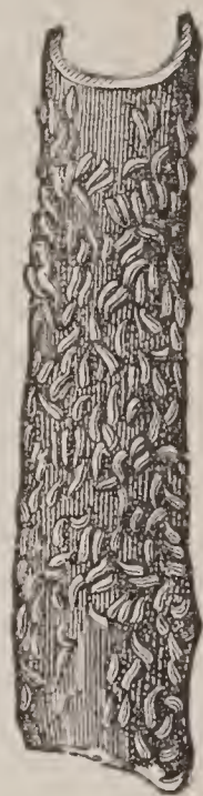
FIG. 336. Oyster-shell bark-louse.
