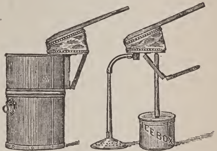
FIG. 401. — Milk Aerator.
